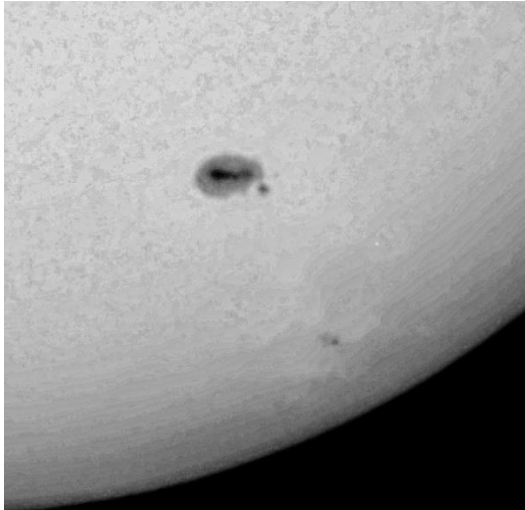
Close up of the active regions on May 20 th
